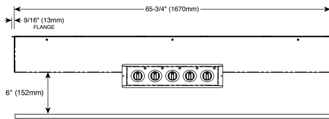
Optional stainless steel heat shield (not factory supplied)
